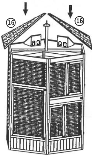
5. Fix the two bars then insert it.
