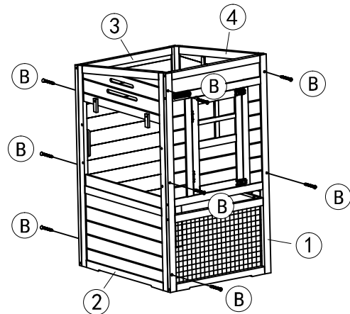
2. Fix the front panel and the left panel with the back panel and the middle partition.
