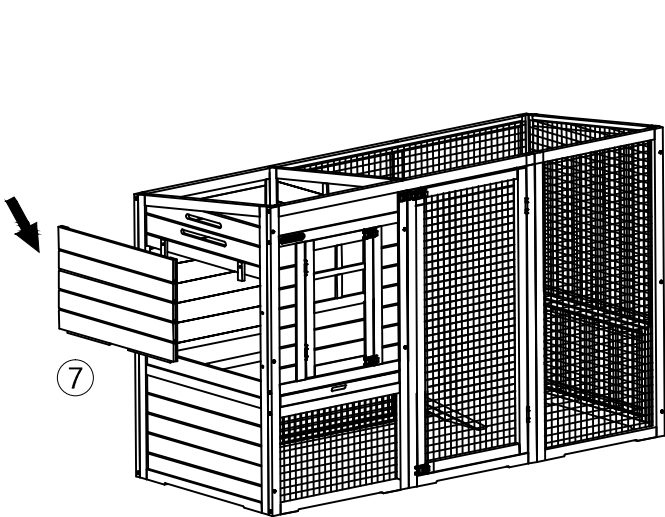
7. Insert the detachable door.
