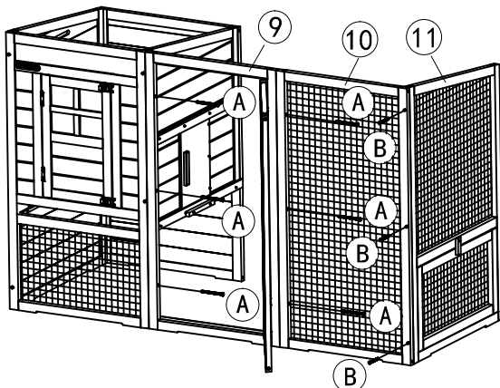
3. Fix the enclosure left & right front panel with enclosure side panel.
