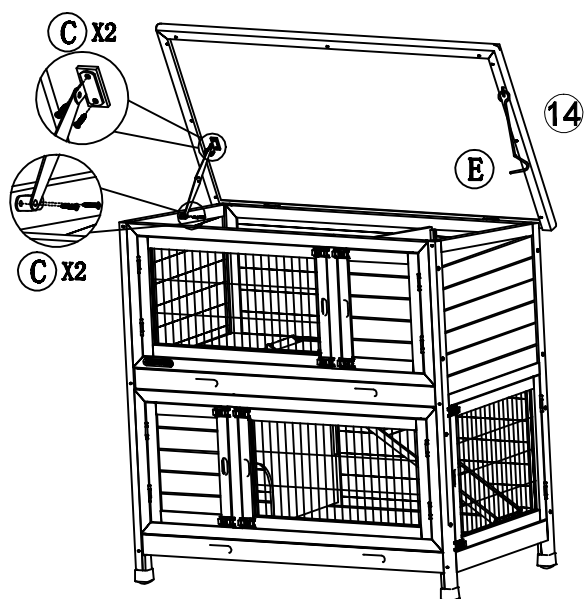
9. Fix the hinge.
