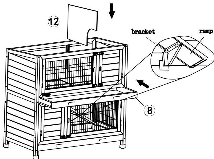
5. Fix the bottom tray and the partition.
