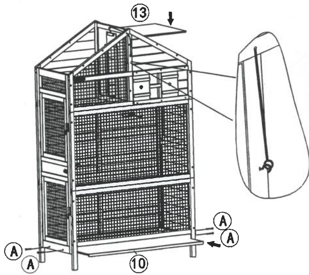
5. Fix the bottom panel and the shelf, and then fix the ring on the line.
